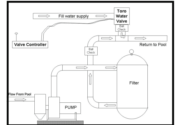
Diagram of One possible Remote Valve Location
